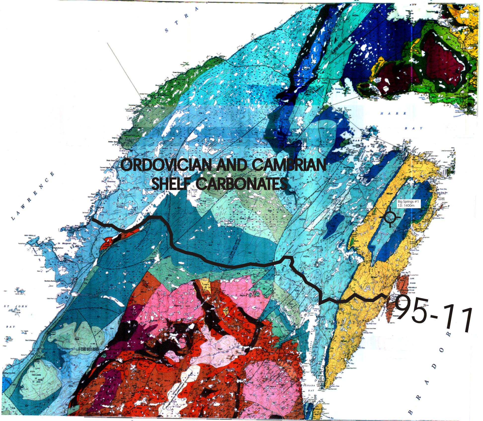
MAP 1495A GEOLOGY STRAIT OF BELLE ISLE AREA NORTHWESTERN INSULAR NEWFOUNDLAND, SOUTHERN LABRADOR AND ADJACENT QUEBEC
